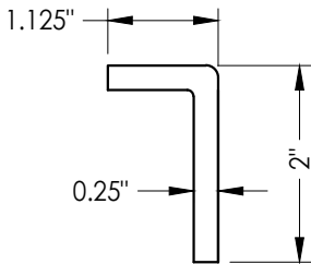
3 ASTRAGAL (FRP)
